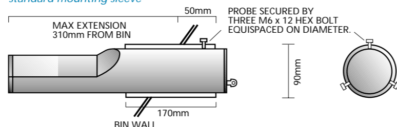
Hydro-Probe II fitted with standard mounting sleeve
